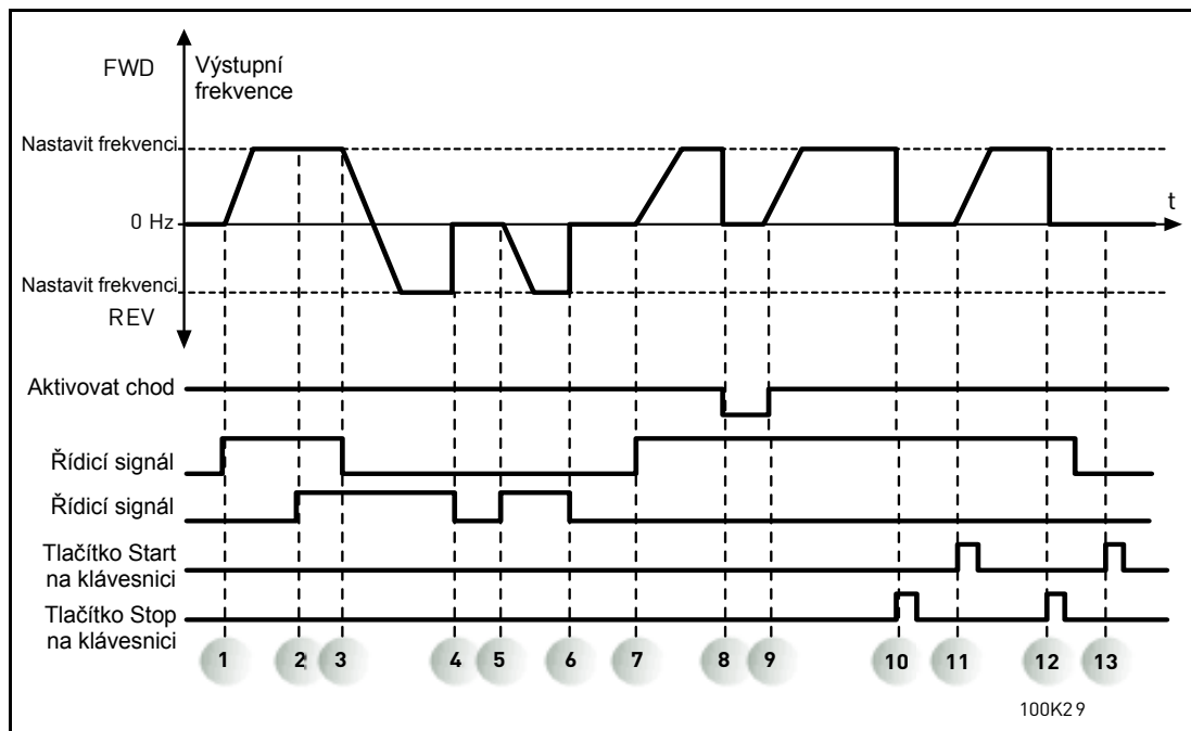
Obr. 18. Start/Stop logika I/O A = 0
