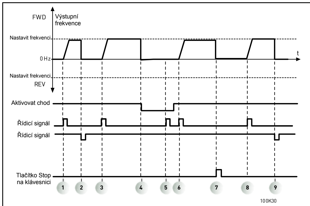
Obr. 19. Start/Stop logika I/O A = 1
