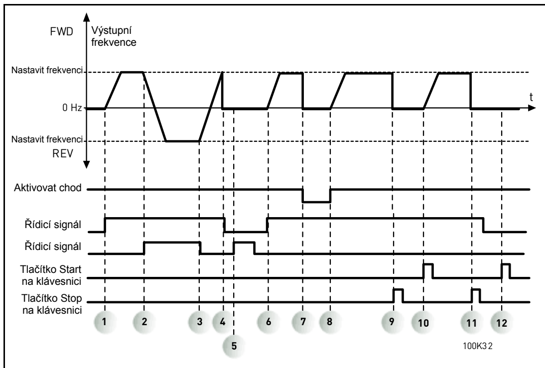
Obr. 21. Start/Stop logika I/O A = 3
