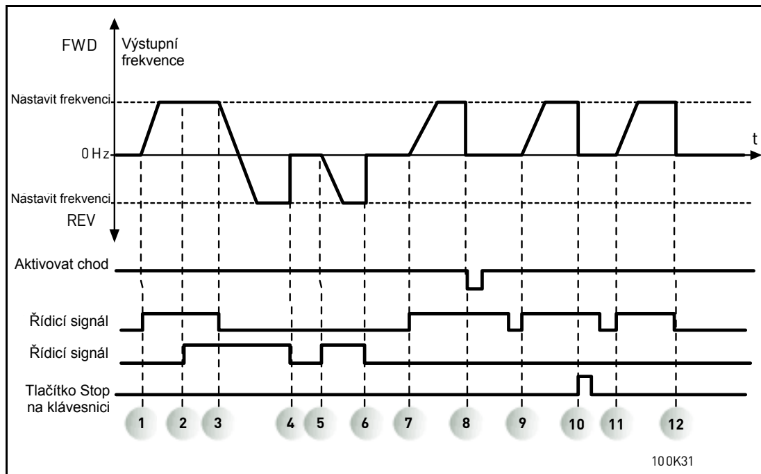
Obr. 20. Start/Stop logika I/O A = 2
