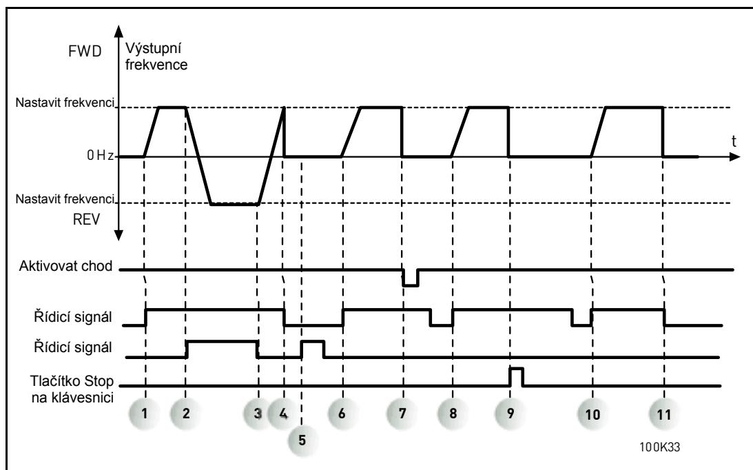
Obr. 22. Start/Stop logika I/O A = 4
